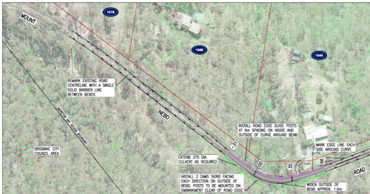
Figure - Concept plan of proposed black spot project at #1044 Mt Nebo Road
